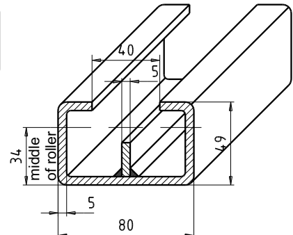
High profile guide weight: 8,1 kg/m
