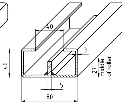
Low profile guide weight: 4,8 kg/m
